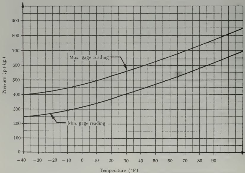
FIGURE 9-21. Fire extinguisher container pressure-temperature curve.
